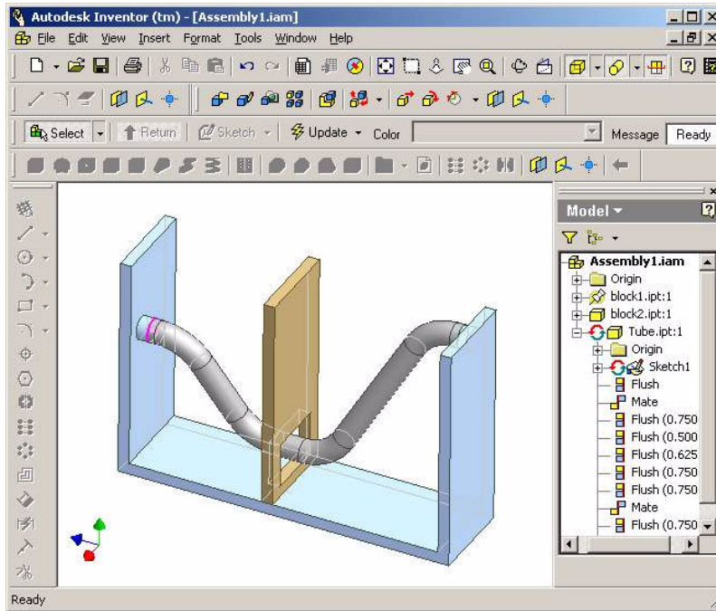
Figure 8 - Moving the Cutout Changes Hose Geometry
