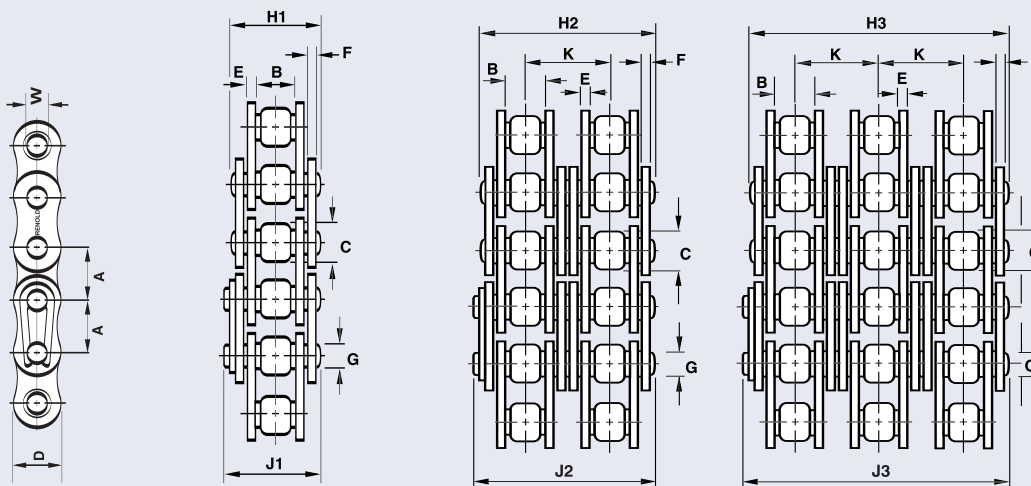
Chain Technical Details (mm) Connecting Links
